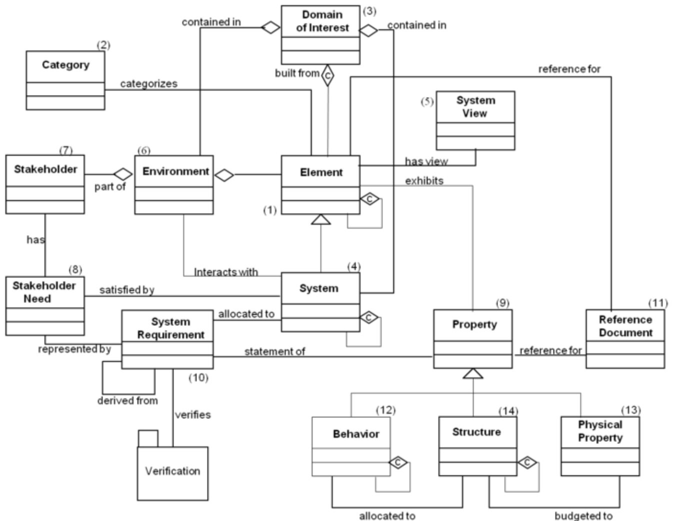
Figure 1. Fragment of the Object Management Group System Concept Model (Oliver 2003, Slide 3). Permission granted by David Oliver on behalf of INCOSE MDSW Working Group. All other rights are reserved by the copyright owner.
