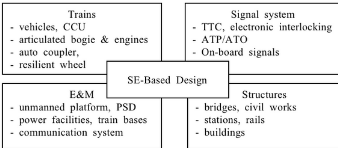
Figure 1. Subsystems of the SKLTS (Ahn, 2005). (Notes: CCU: Central Control Unit; TTC: Total Traffic Control; ATP: Automatic Train Protection; ATO: Automatic Train Operation; PSD: Platform Screen Door) Reprinted with permission of Journal of the Korean Society for Railway . All other rights are reserved by the copyright owner.
